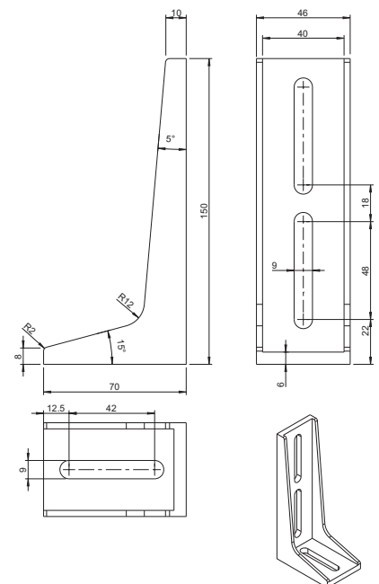
Support bracket 03
