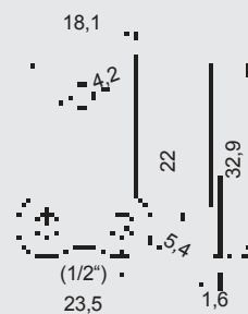
For chain L 85 SL: Design 120.11
