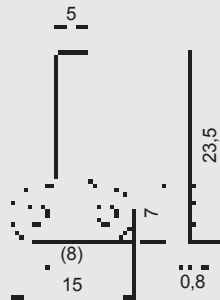
For chain G 52: Design 121.0
